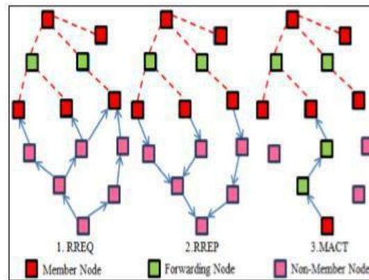
Figure 2: MAODV Protocol
